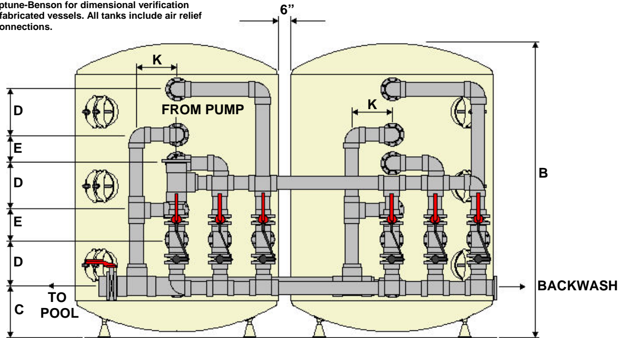
Model DTC
