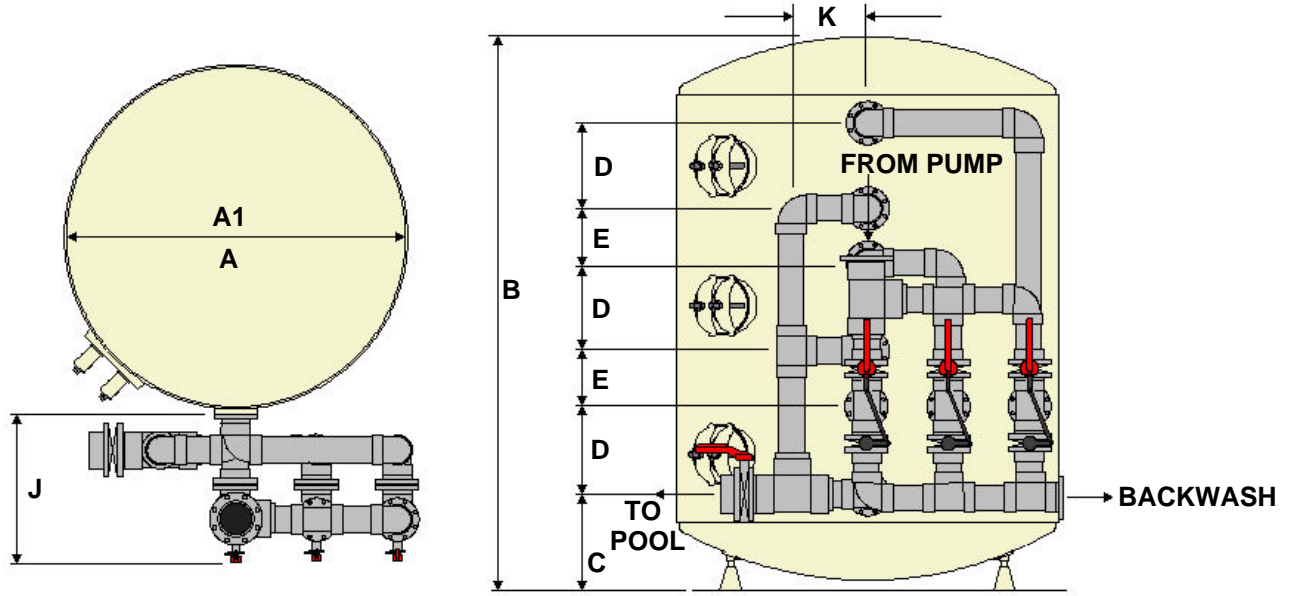
Model STC
