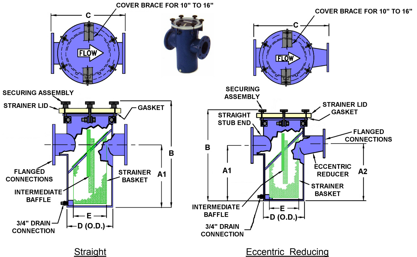
Capacity And Dimension Chart
